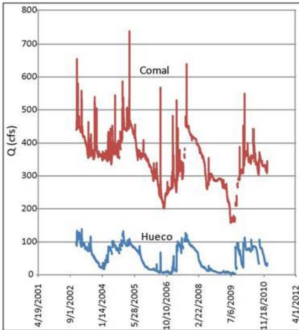
Figure 4-40. Hydrographs of Comal and Hueco Springs, 2002 to 2010
