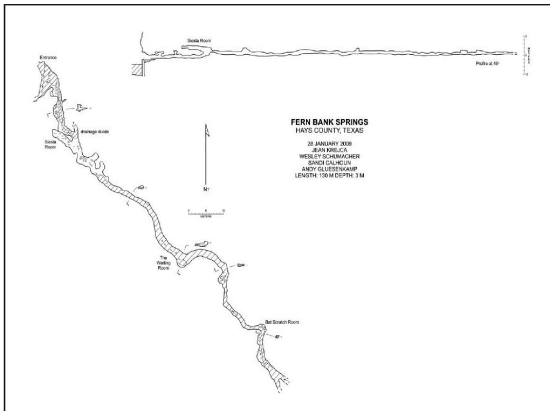
Figure 3-14. Cave Map of Fern Bank Springs
