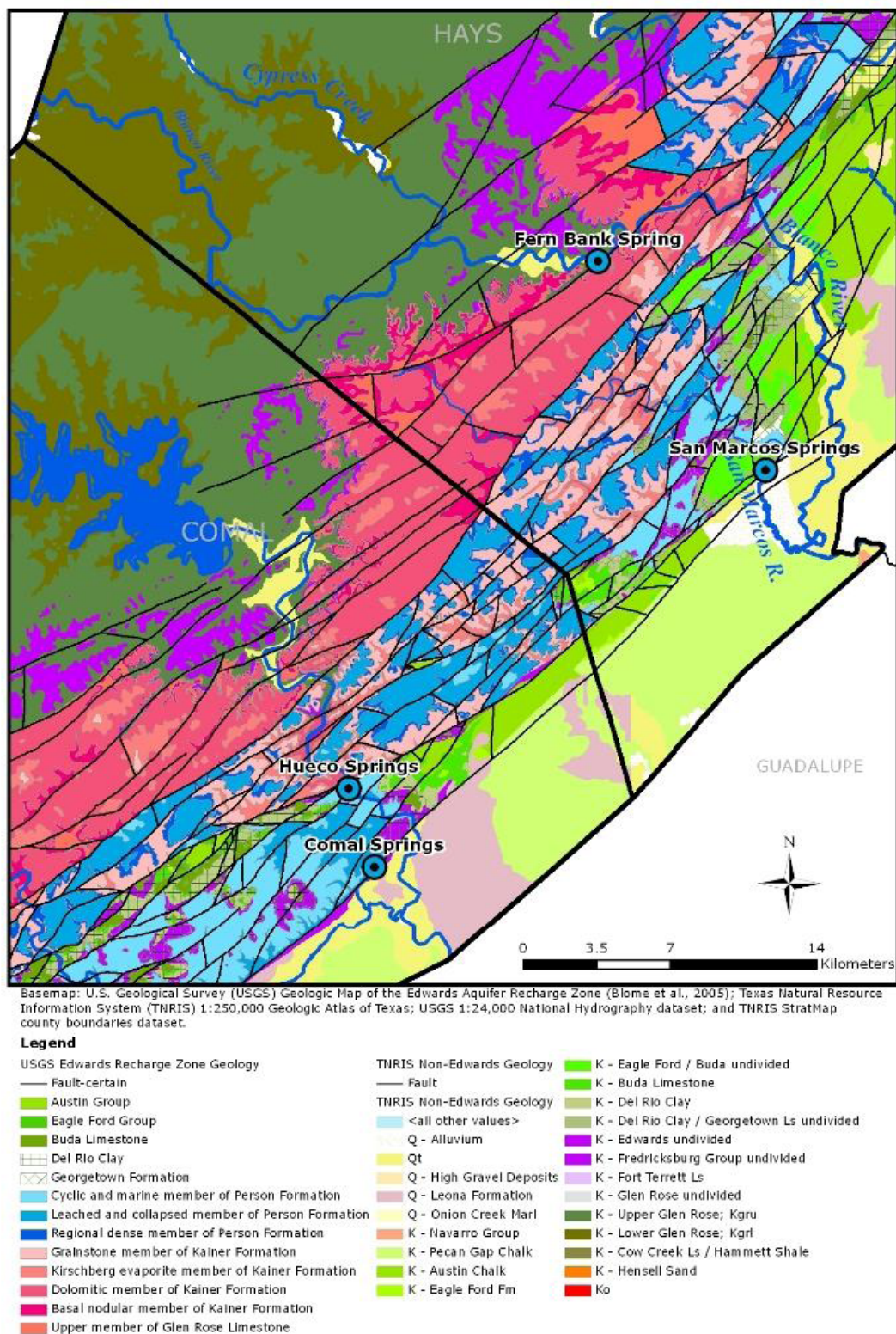
Figure 4-39. Location and geology surrounding springs
