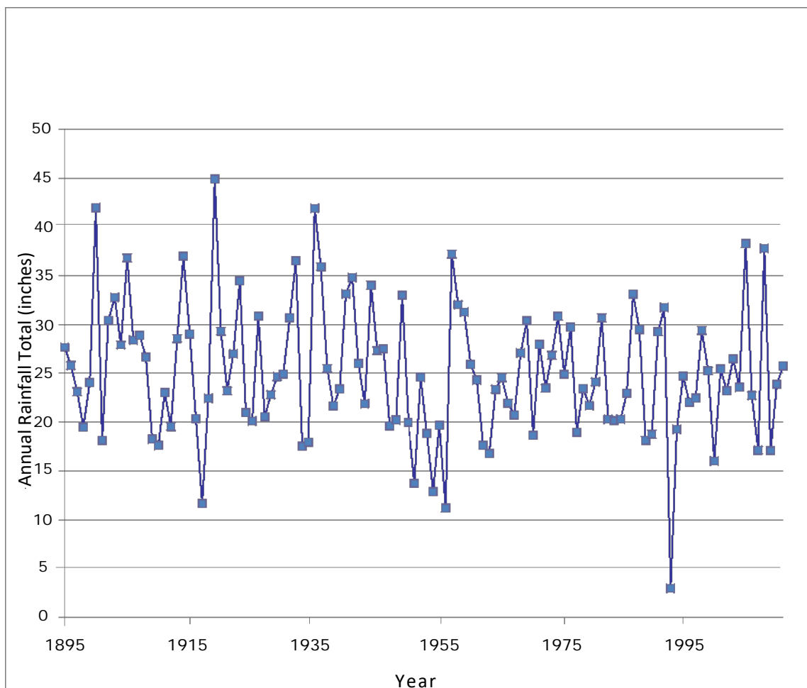
Figure 3-5. Division 6 Rainfall
