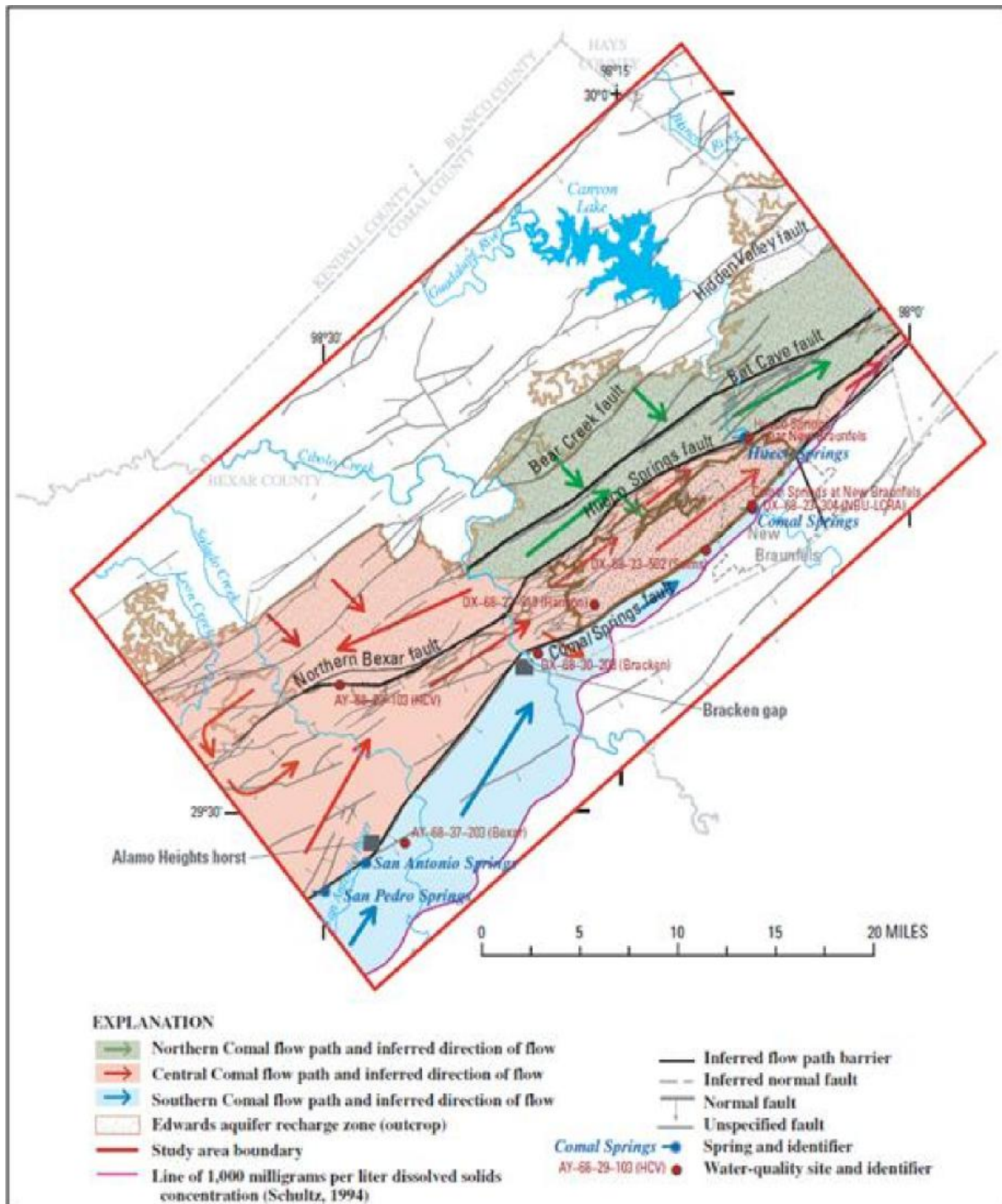
Figure 3-13. Major Faults and Interpreted Groundwater Flowpaths to Comal and Hueco Springs from Otero (2007)
